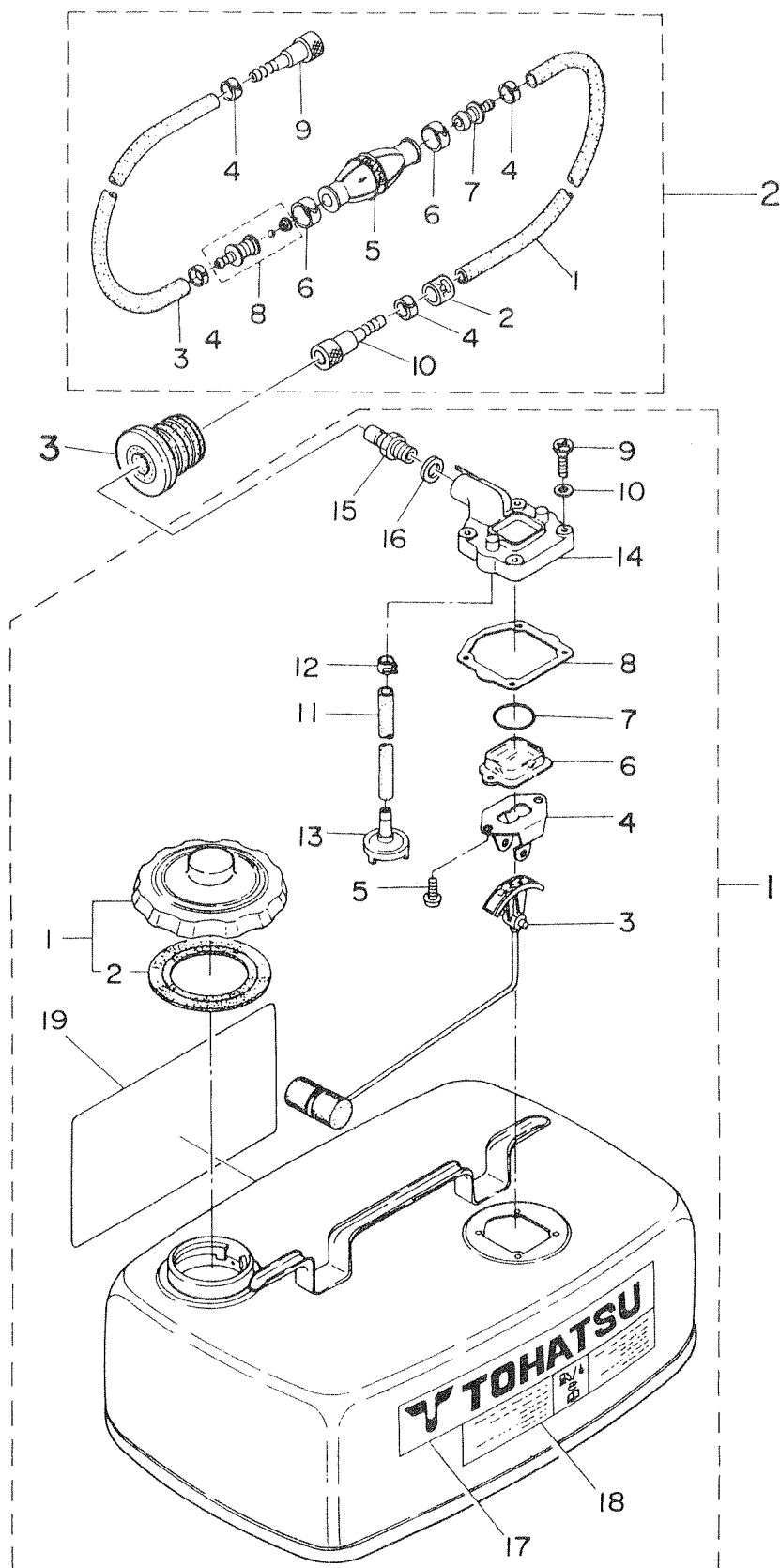
Fig. 26-A OPTIONAL PARTS (III) ACCESSORIES (3) AUTO AIR VENT
